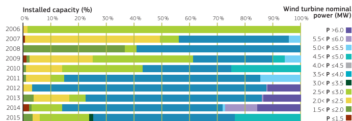
Figure 7: Change in nominal power of offshore wind turbines in the world. Source: JRC wind energy database.
