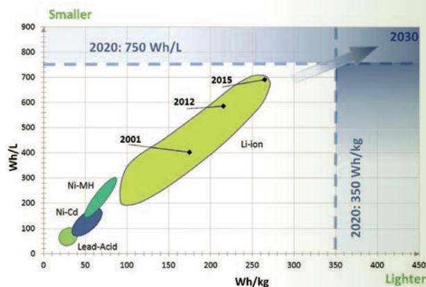
Figure 19: The energy density of Li-ion batteries has been increasing steadily over recent years.
