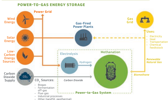
Figure 22: Electrochaea power-to-gas system.
