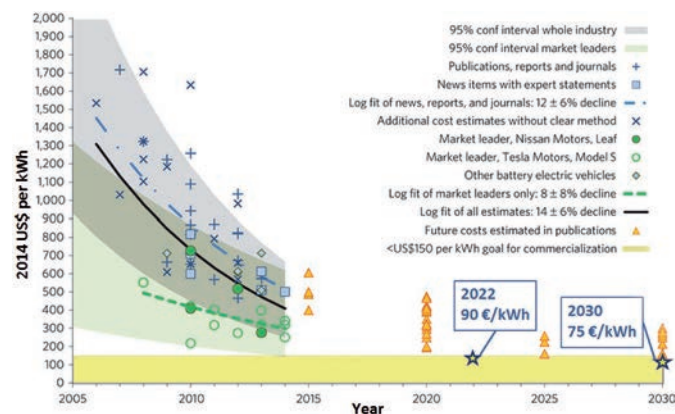
Figure 20: The cost of Li-ion battery packs in battery electric vehicles has fallen dramatically over recent years.
